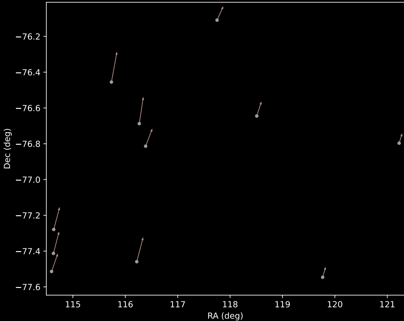
GALAH DR4 Cluster 11 Proper Motion Vectors (n=11)
