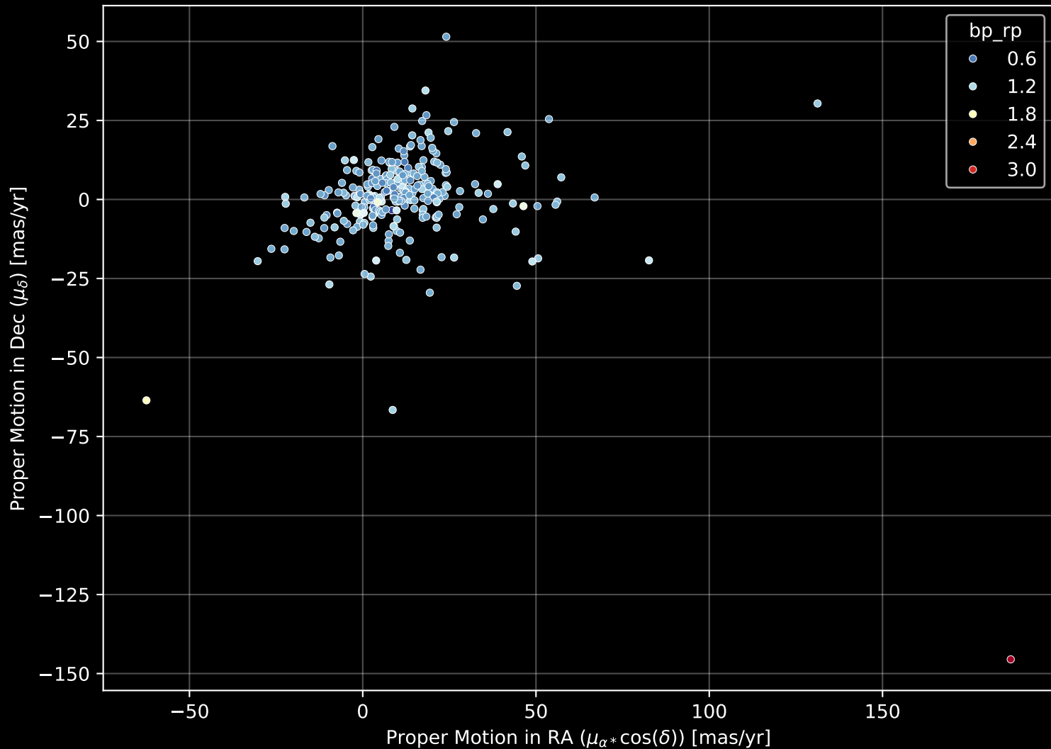
GALAH DR4 Field: [202] Proper Motion Diagram (n= 288)
