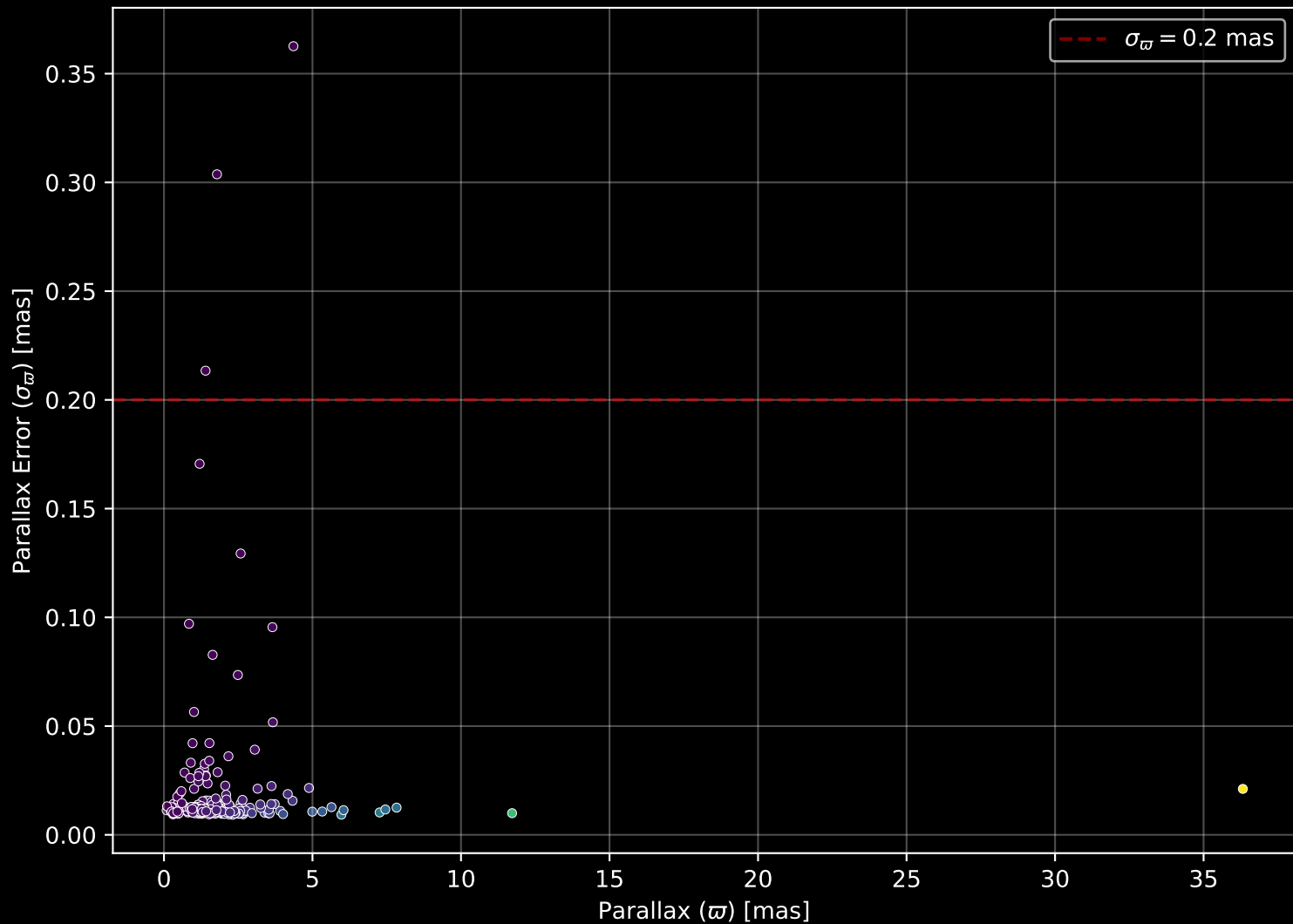
GALAH DR4 Field: [202] Parallax Quality (n= 288)
