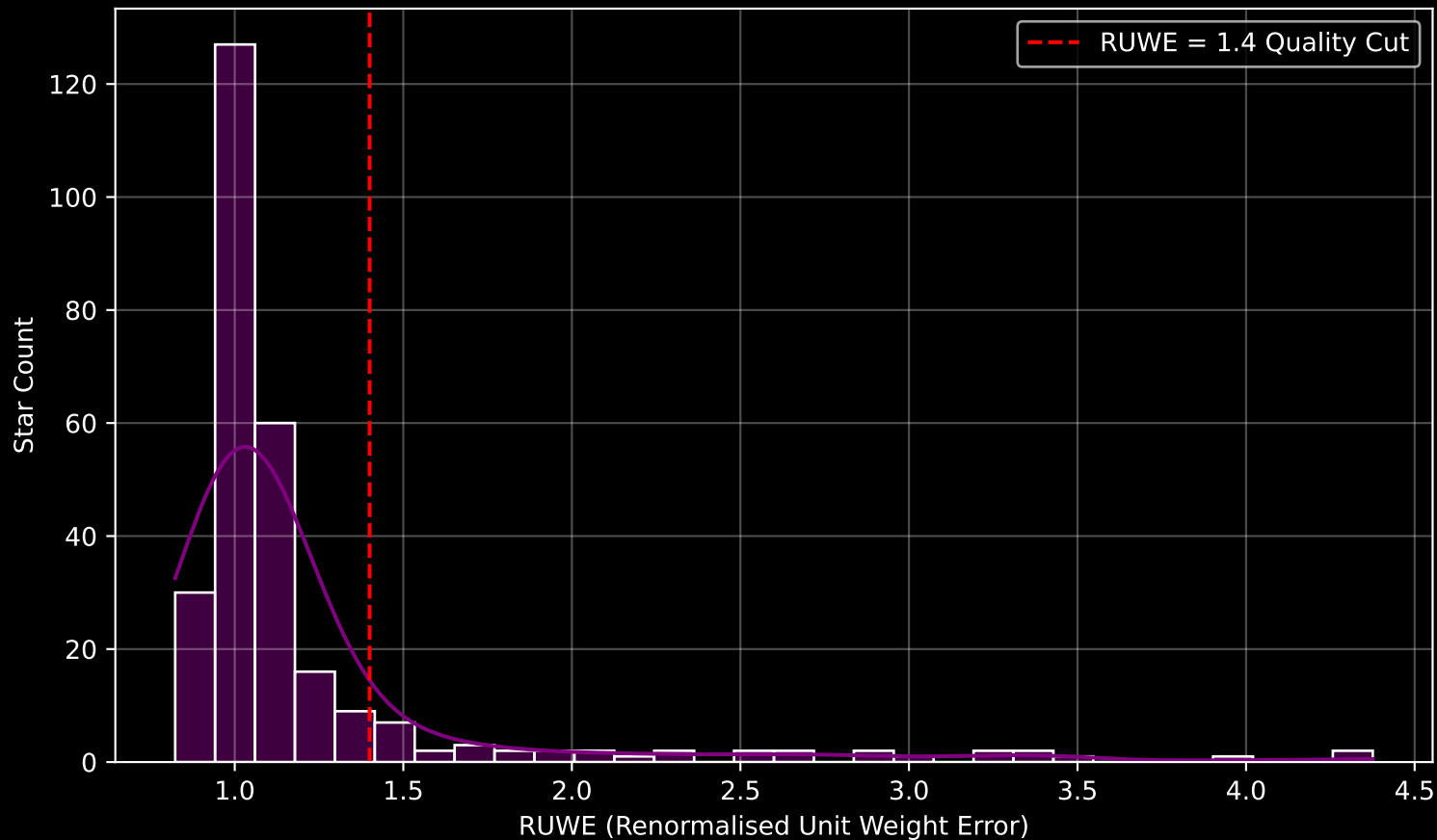
GALAH DR4 Field [202] RUWE Distribution (n= 278)
