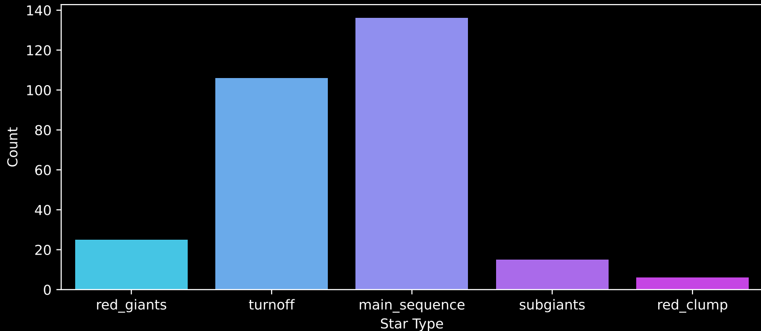
GALAH DR4 Field: [202] Count plot of Star Type
