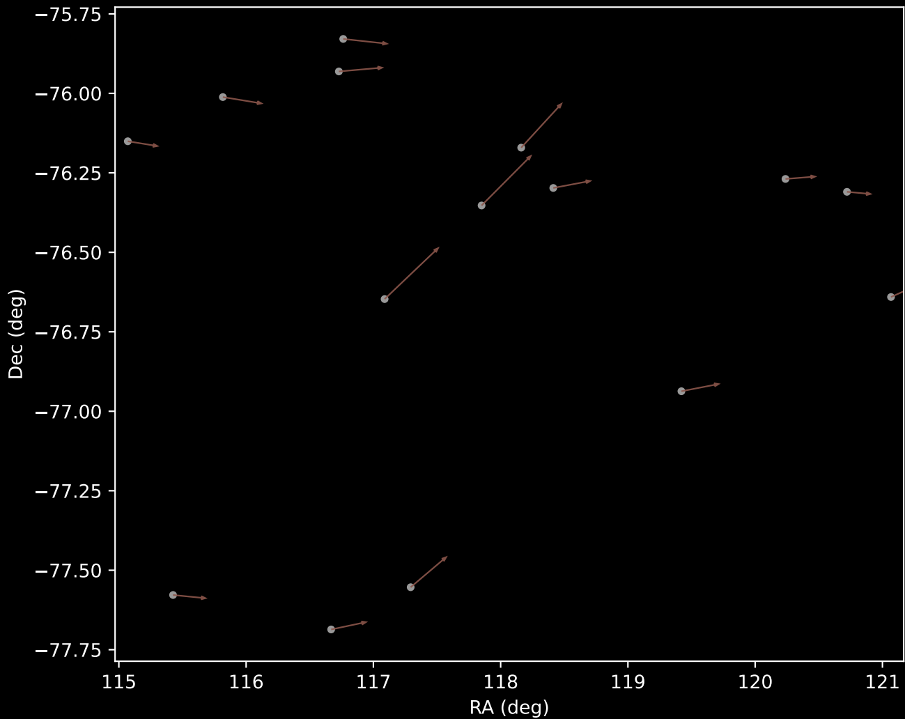
GALAH DR4 Cluster 10 Proper Motion Vectors (n=15)
