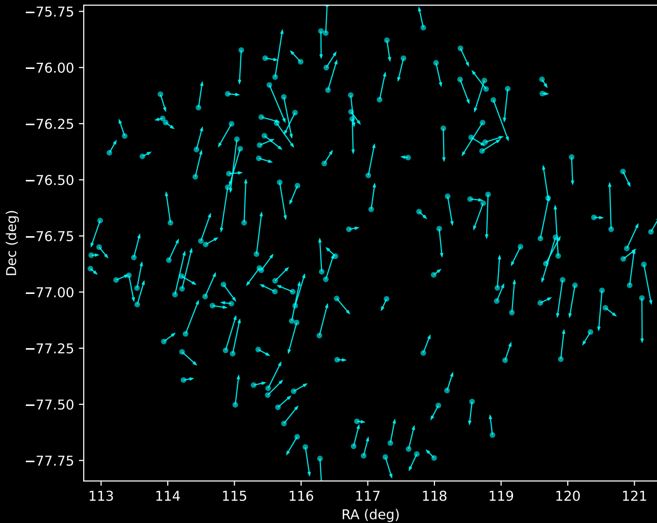
GALAH DR4 Noise Stream Proper Motion Vectors (n=160)
