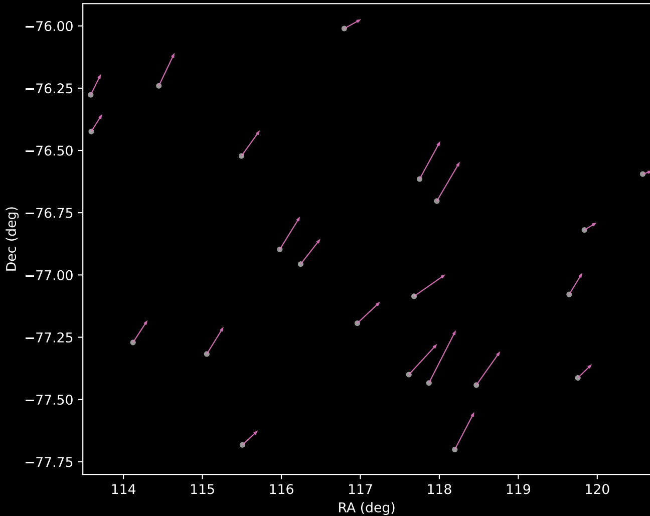
GALAH DR4 Cluster 12 Proper Motion Vectors (n=22)
